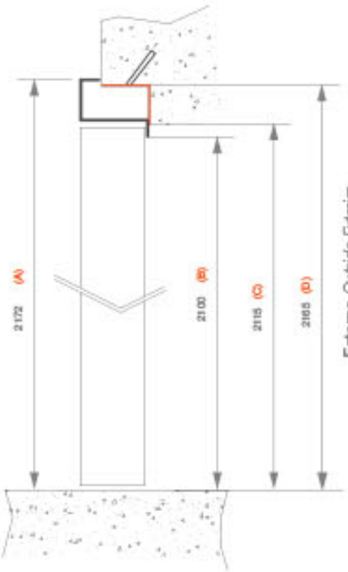
Montato a filo interno Installation flush with internal wall Instalado a raz del revoque interno
